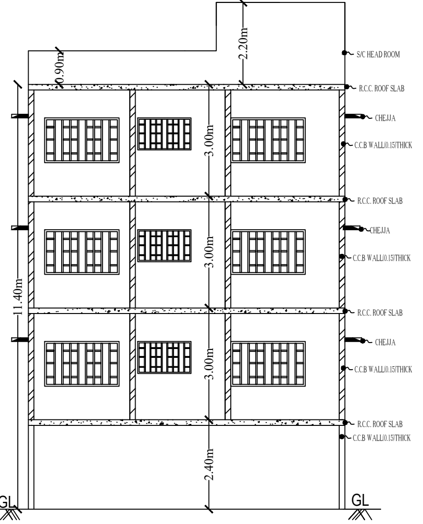
SECTION @ A-A'
